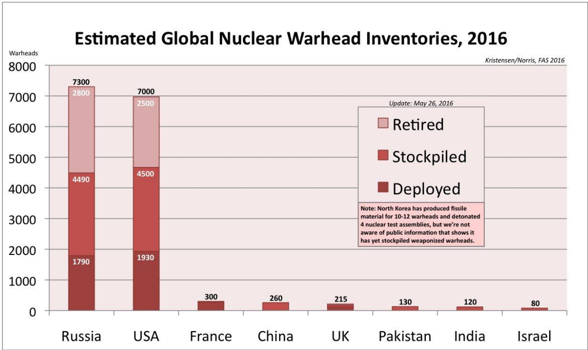
Figure 10.11: Estimated Nuclear Weapons Inventories, 2016
